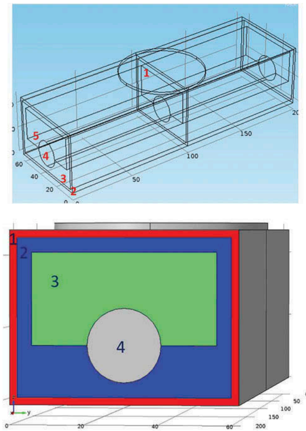
Figure 1. Geometry used in the numerical simulations for the transversal mode. Region 1 is the active electrode for the transversal simulations. Region 2 has the physical properties of skin. Region 3 has the physical properties of fat. Region 4 has the physical properties of bone, and region 5 has the physical properties of muscle.
